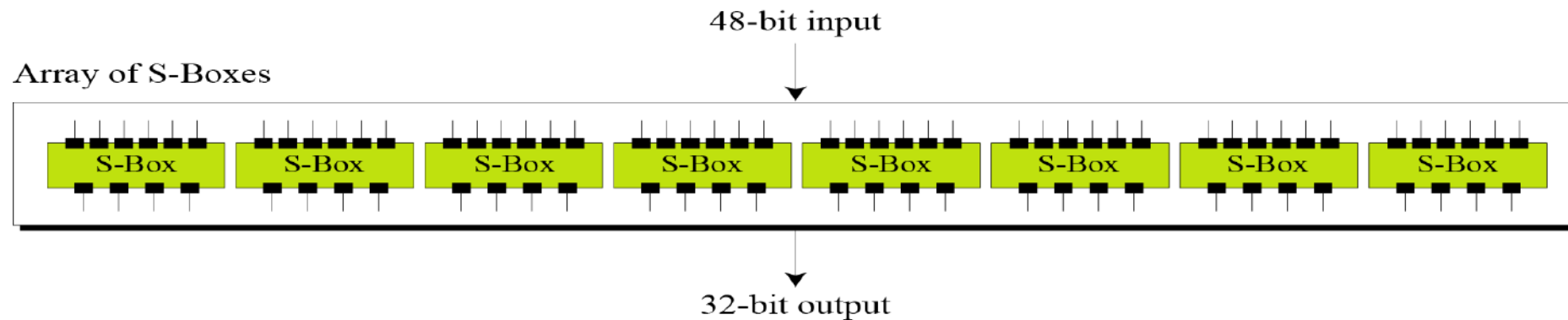
Figure 6.7 S-boxes
